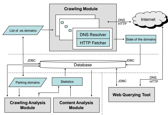
Figure 1: Crawler architecture.
